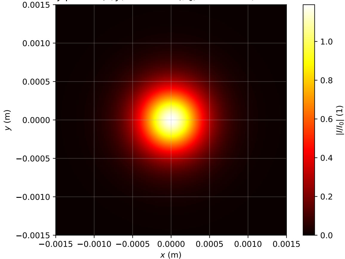
Intensity profile I(x, y, z = 2.627m)/I_0 , P_{in}=0.8P_{cr} , artificial time
